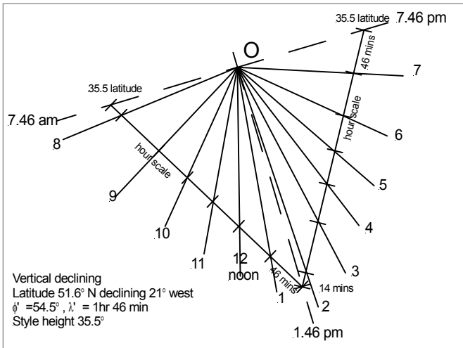
Fig. 5. Vertical dial declining 21° west, latitude 51.6° N. Designed using the calculators in figs 1 and 2 and dialling scales.
