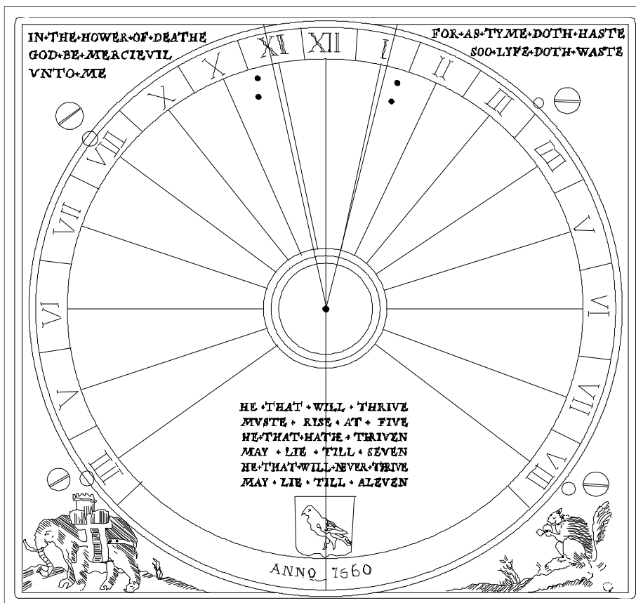
Fig. 5. Line drawing of the Norfolk dial plate by the author.
