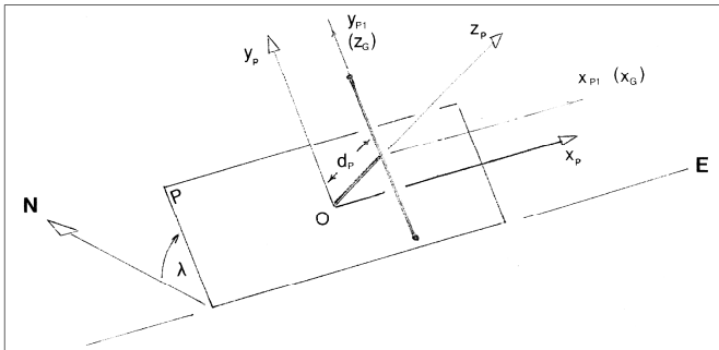
Fig. 19. Polar dial. Axis system.
