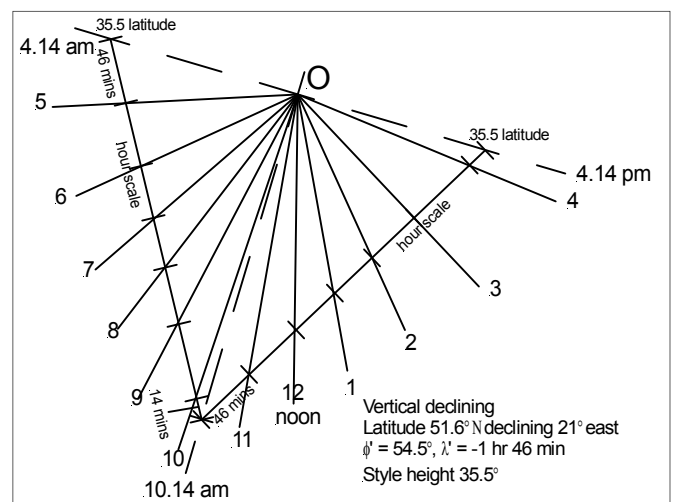
Fig. 4. Vertical dial declining 21° east, latitude 51.6° N. Designed using the calculators in figs 1 and 2 and dialling scales.
