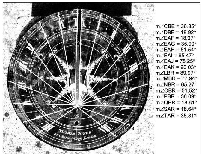
Fig. 2. The dial plate plus hour angles.
