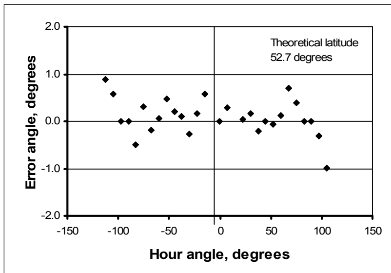
Fig. 9. Analysis of the accuracy of the hour lines.
