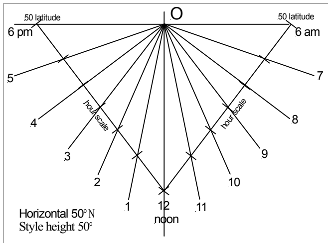
Fig. 3. Horizontal dial 50° N, drawn with dialling scales.
